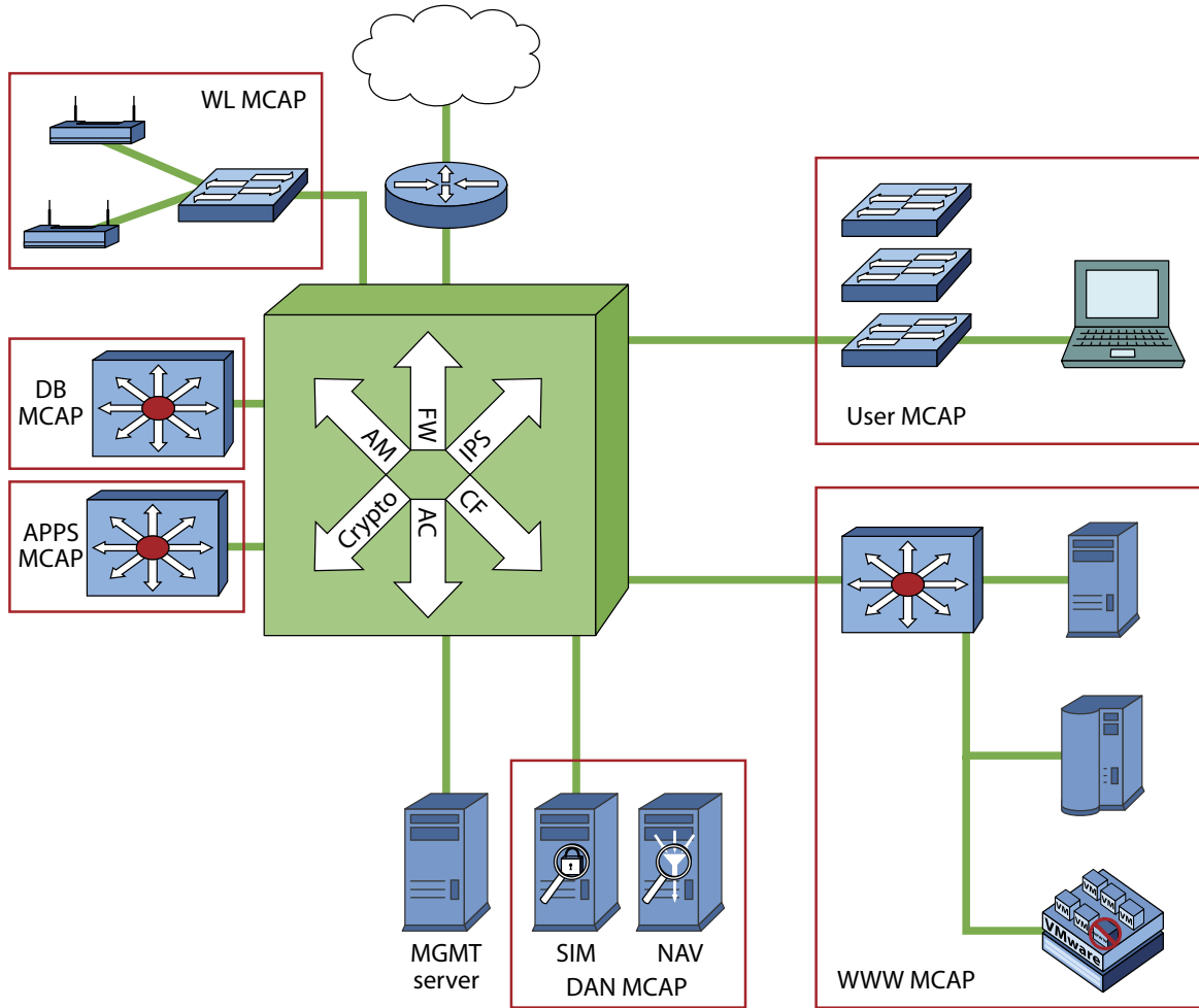
Figure 9 Zero Trust Network Architecture Is Scalable
