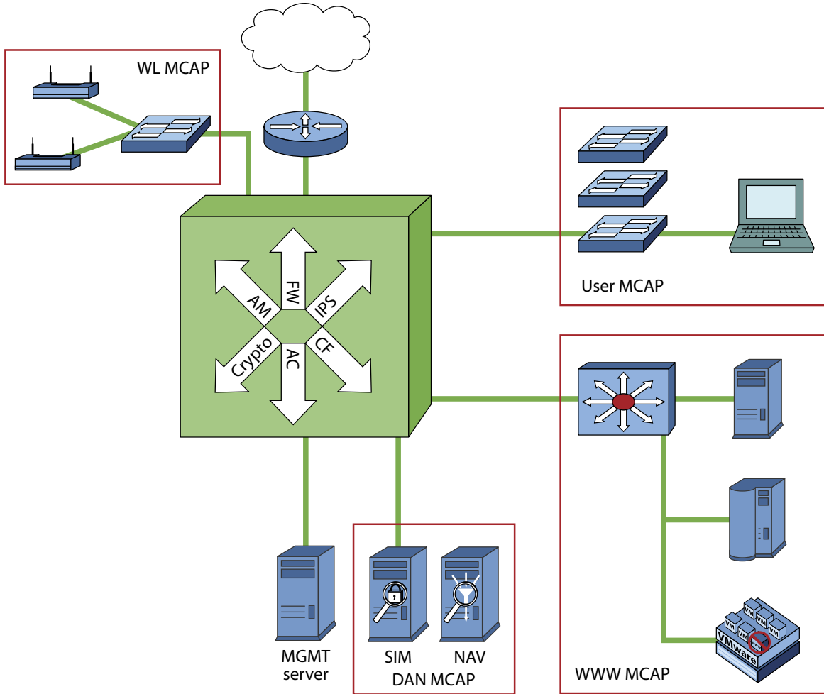
Figure 8 Zero Trust Network Architecture Is Compliant
