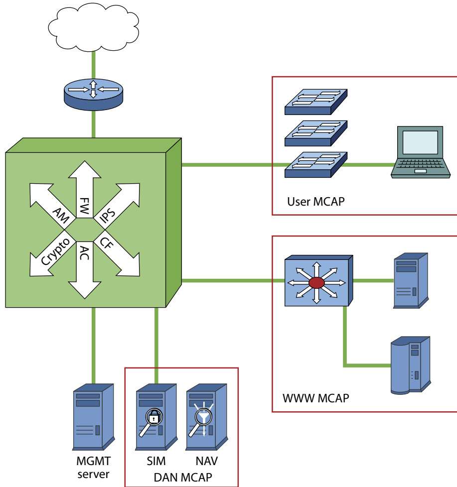
Figure 6 Zero Trust Is Platform-Agnostic
