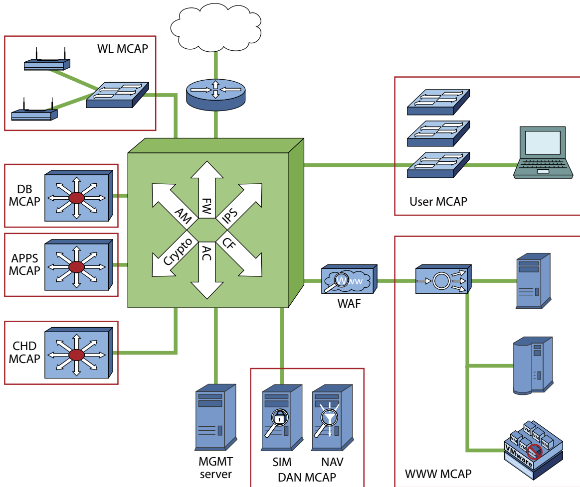
Figure 12 Zero Trust Network Architecture Is Extensible
