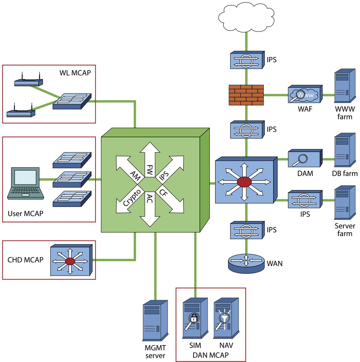
Figure 13 Augment Hierarchical Networks With Zero Trust
