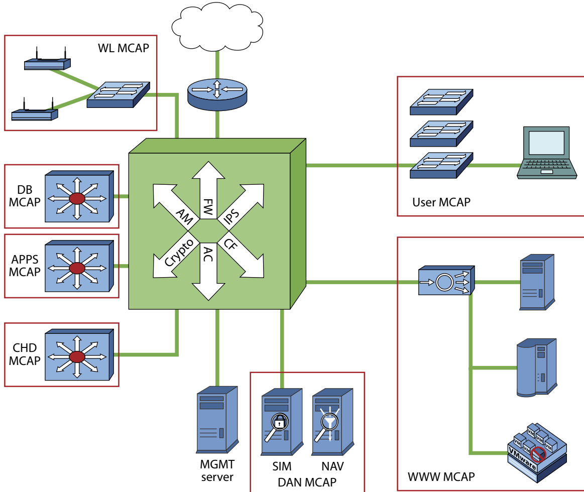
Figure 11 Zero Trust Network Architecture Is Flexible
